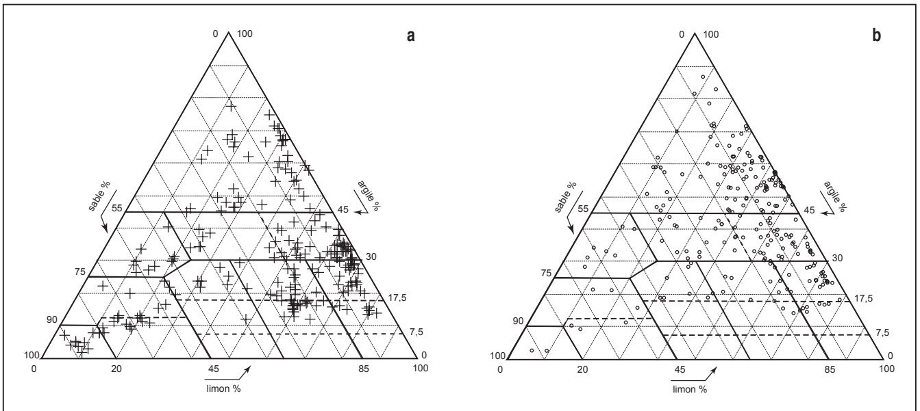
Figure 2 – Texture of the horizons used to establish the class pedotransfer functions (CPT) (a) and of those used to test their validity (b).
