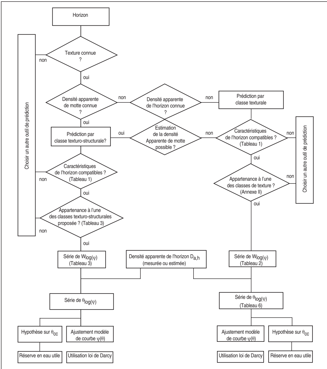
Figure 4 – Flowchart illustrating the estimation method of the water retention properties for an horizon.
