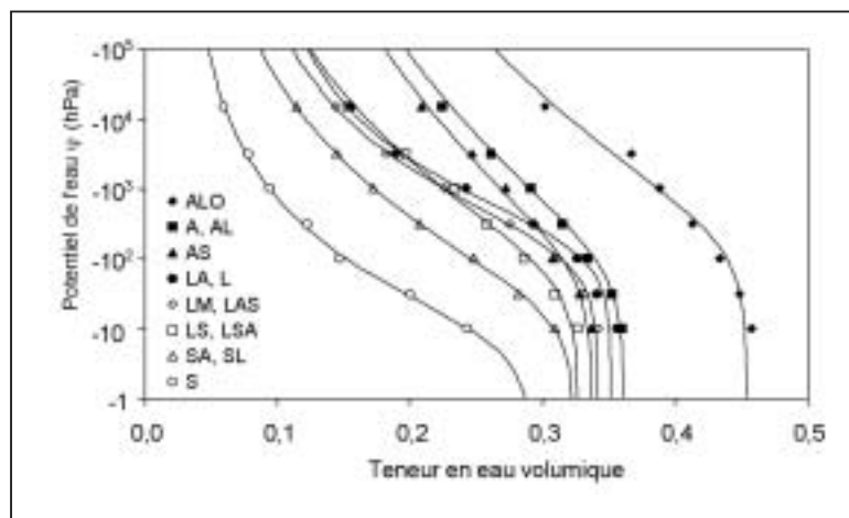
Figure 3 – Mean volumetric water contents proposed after textural stratification with respect to values of horizon bulk density ( D_{a,h} ) that were similar to D_{a,m}^* round down to the tenth lower (table 6) and adjusted curves using the van Genuchten's model (parameters are given in table 8).
